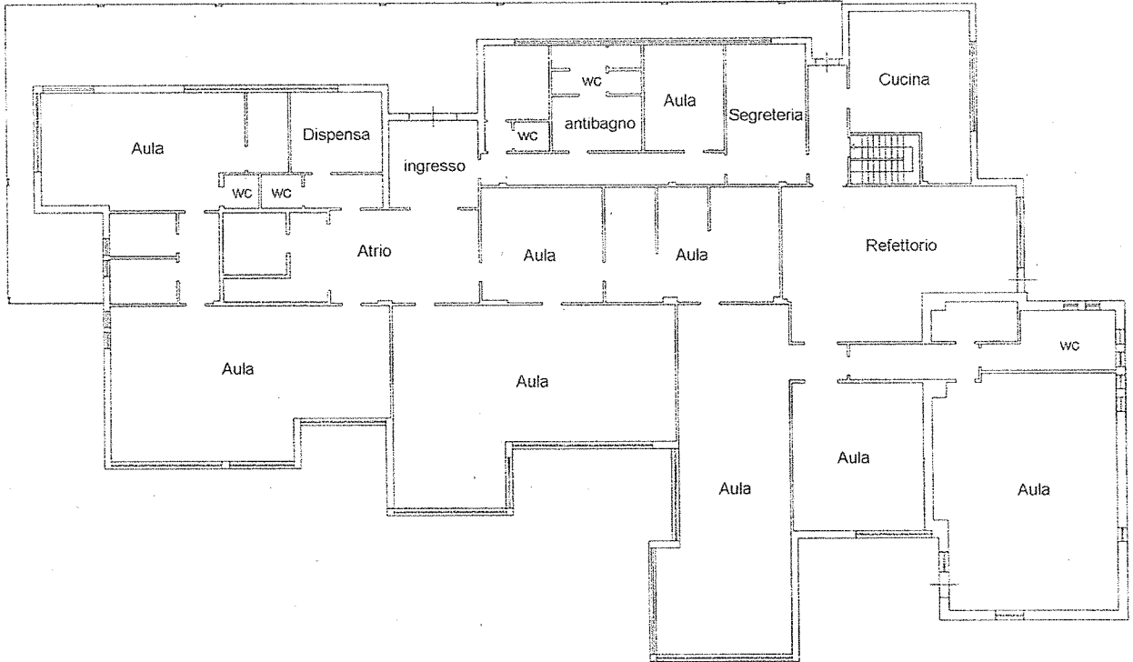
PIANO TERRA
